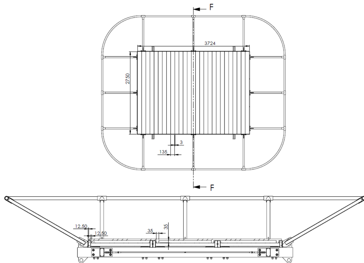
SECTION F-F
